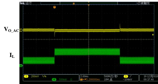
Load Transient
