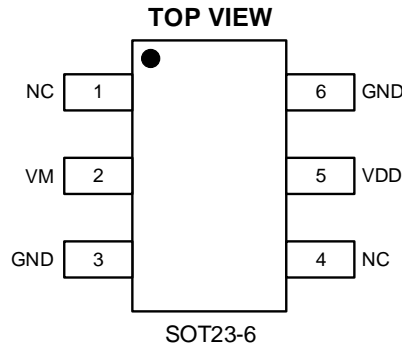
Figure 2. Pin Configuration
